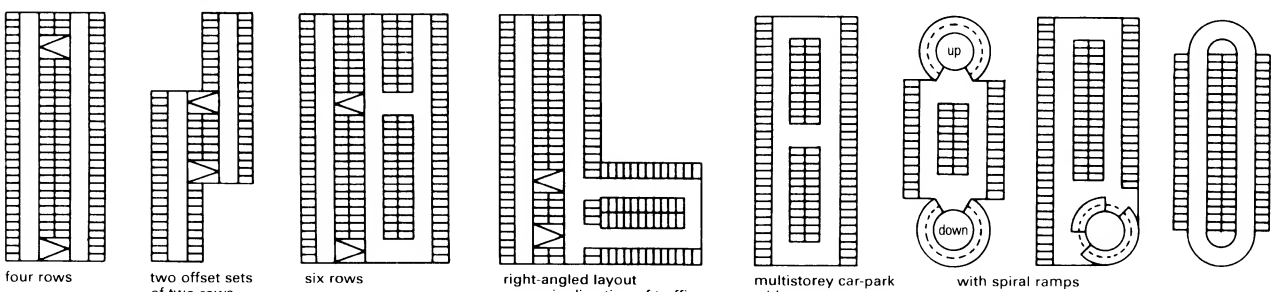
⑦ Plan views and arrangement of ramps
